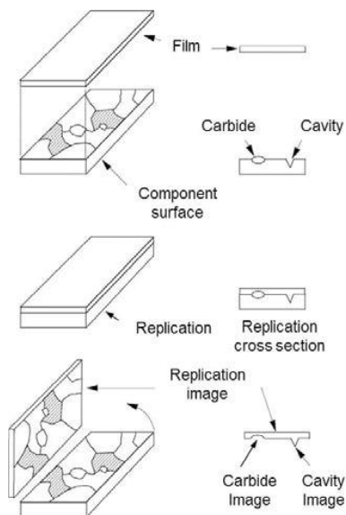
Fig. 2 Schematic representation of the plastic replica technique [8]
