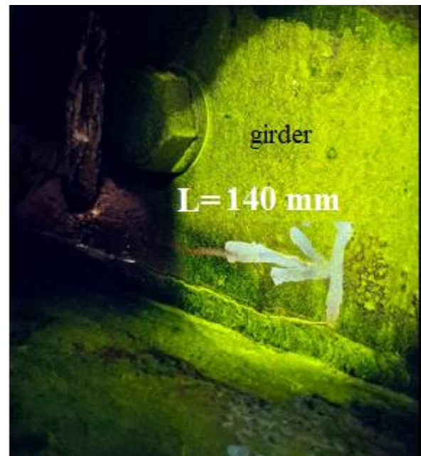
Fig. 4 A fatigue crack in the heat affected zone of a steel girder under an orthotropic plate
