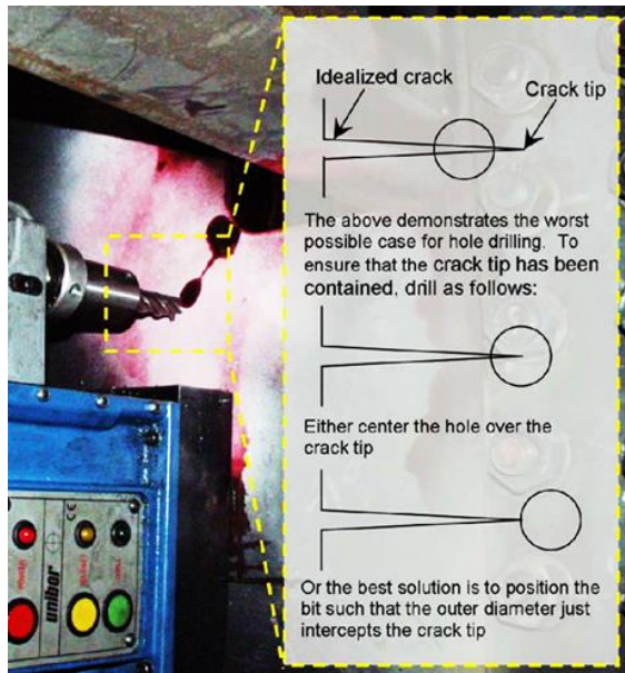
Fig. 8 Correct placement of the drill bit and removal of the crack tip identified by red penetrant
