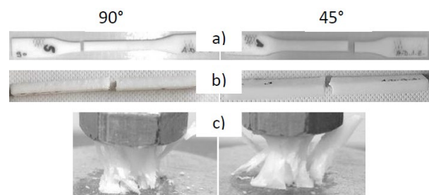
Fig. 2 Fractured specimens printed by DLP-LCD after: a) tensile, b) flexure and c) compression testing
