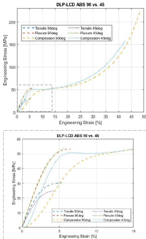
Fig. 5 Stress-strain curves of DLP-LCD printed specimens made of ABS resin in two building orientations
