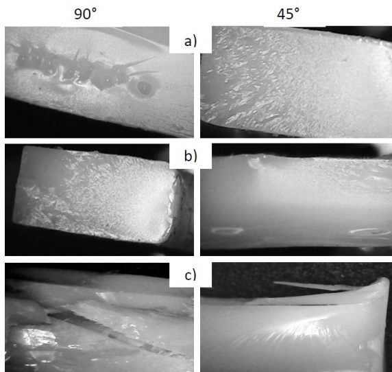
Fig. 3 Fractured surfaces of DLP-LCD printed specimens after: a) tensile, b) flexure and c) compression testing
