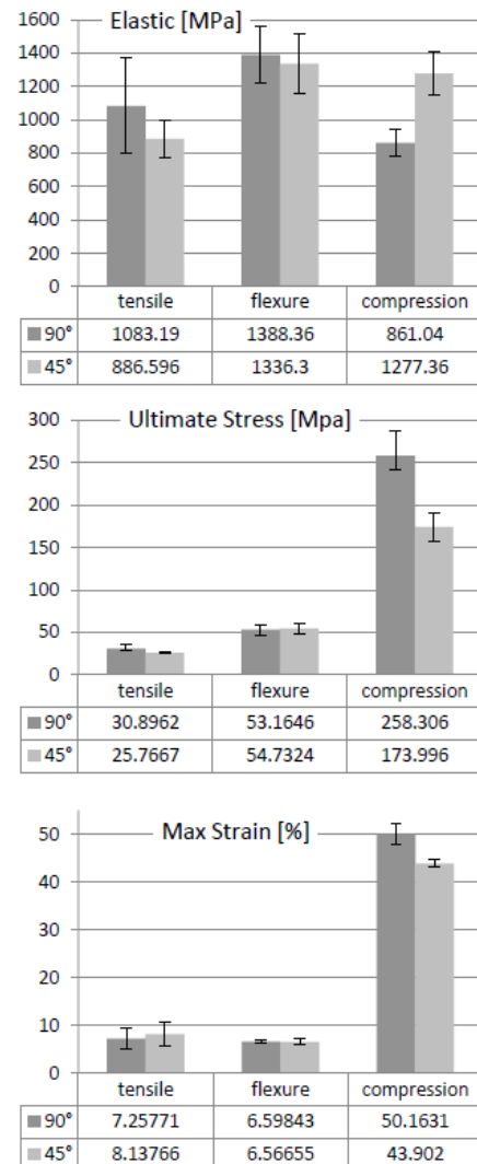
Fig. 4 The main mechanical properties of ABS specimens DLP-LCD printed in two building orientations
