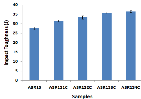
Fig. 7: Impact toughness for the developed hybrid composites
