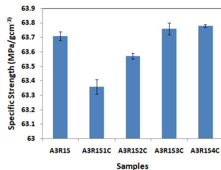
Fig. 6 Specific strength for the developed hybrid composites
